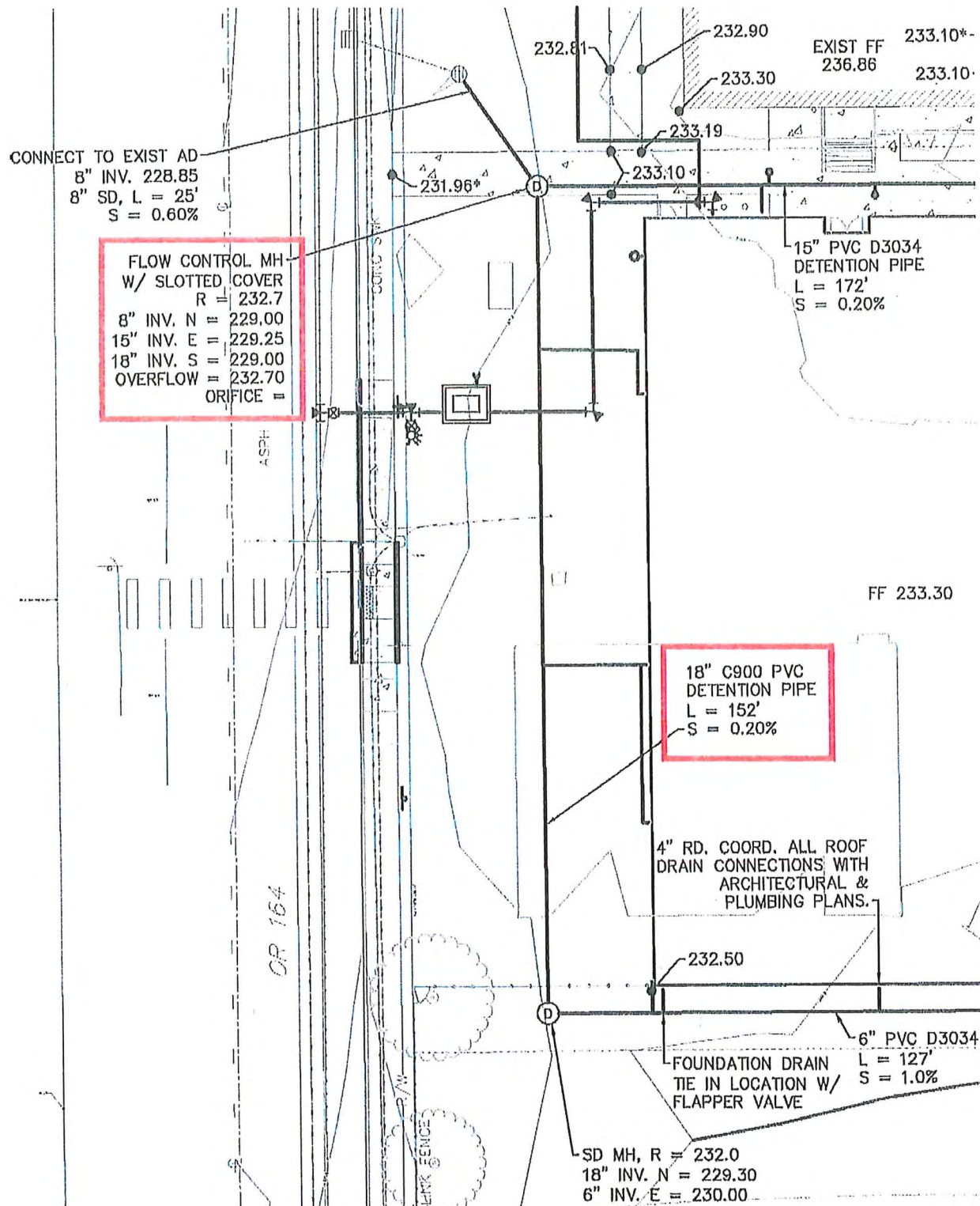
Figure 5-7 | Pipe Detention
